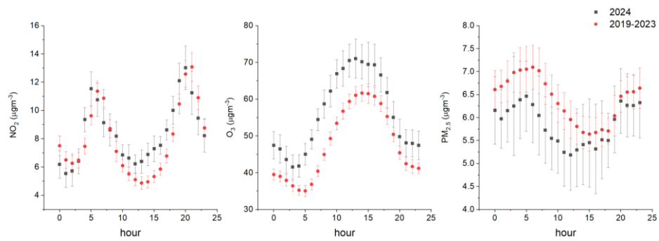
Figure S2: Diurnal variation of NO 2 , O 3 and PM 2.5 measure at BAQS from June to August in 2024 (grey) and in 2019-2023 (red).
