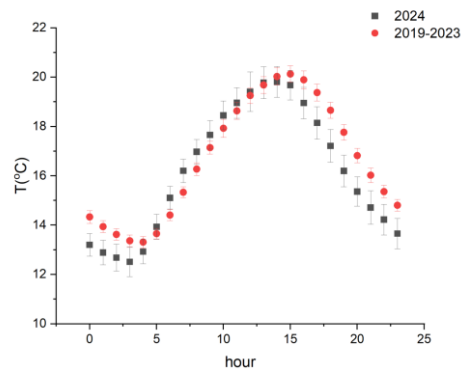
Figure S1: Diurnal variation of temperature measure at BAQS from June to August in 2024 (grey) and in 2019-2023 (red).
